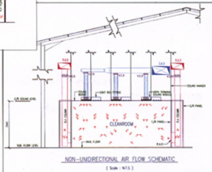
Non-unidirectional air flow cleanroom
