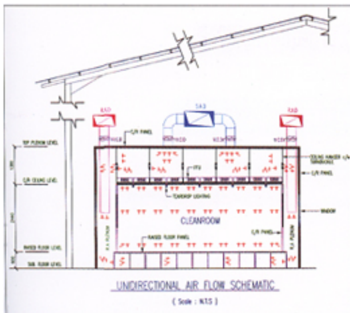
Unidirectional air flow creation
